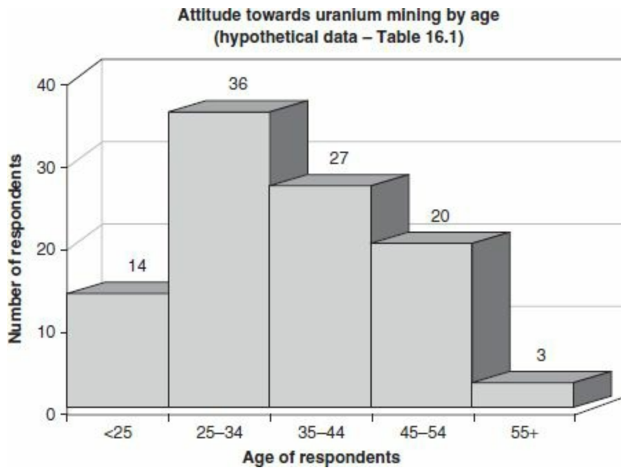
FIGURE 16.2b Three-dimensional histogram
