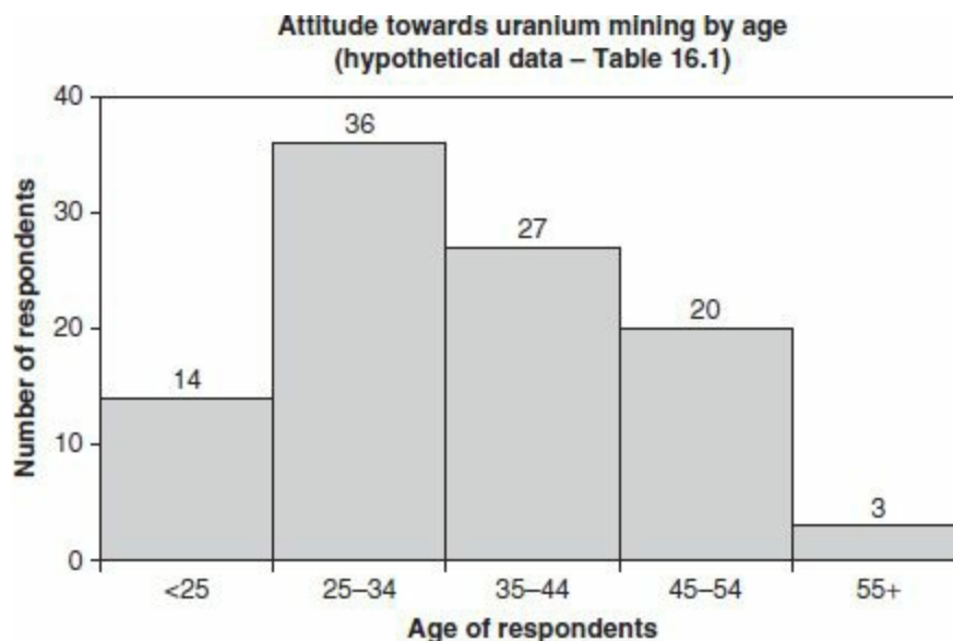
FIGURE 16.2a Two-dimensional histogram
